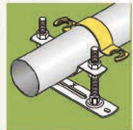
(5) Set the top band by sliding it over the pipe.
