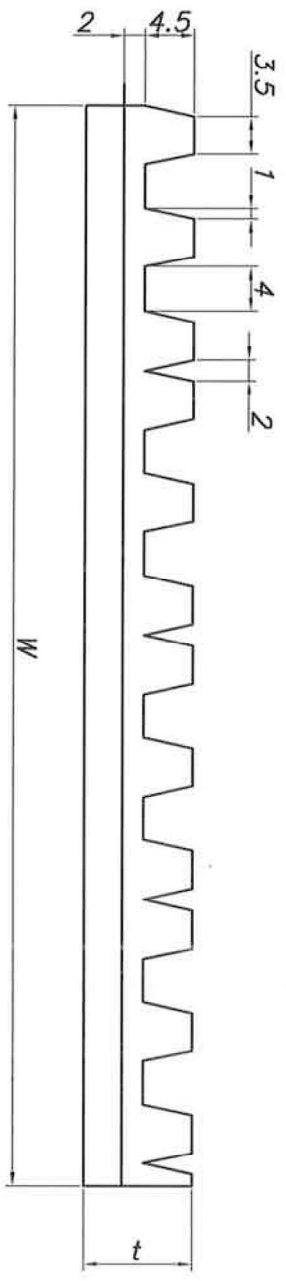
A-A' Sectional view
